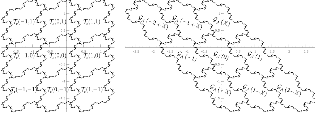
FIGURE 4. The SRS tiles \mathcal{T}_{\mathbf{r}}(\mathbf{z}) for \mathbf{r} = (\frac{1}{2}, -\frac{1}{2}) , \|\mathbf{z}\|_{\infty} \leq 1 , (left) and the Brunotte tiles \mathcal{G}_A(\Psi^{-1}(\mathbf{z})) = V\mathbf{z} + \mathcal{F}_A associated with A = x^2 - x + 2 (right).
