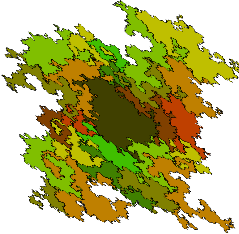
FIGURE 3. The SRS tiles \mathcal{T}_{\mathbf{r}}(\mathbf{x}) with \|\mathbf{x}\|_{\infty} \leq 2 corresponding to \mathbf{r} = (\frac{3}{4}, 1) .
