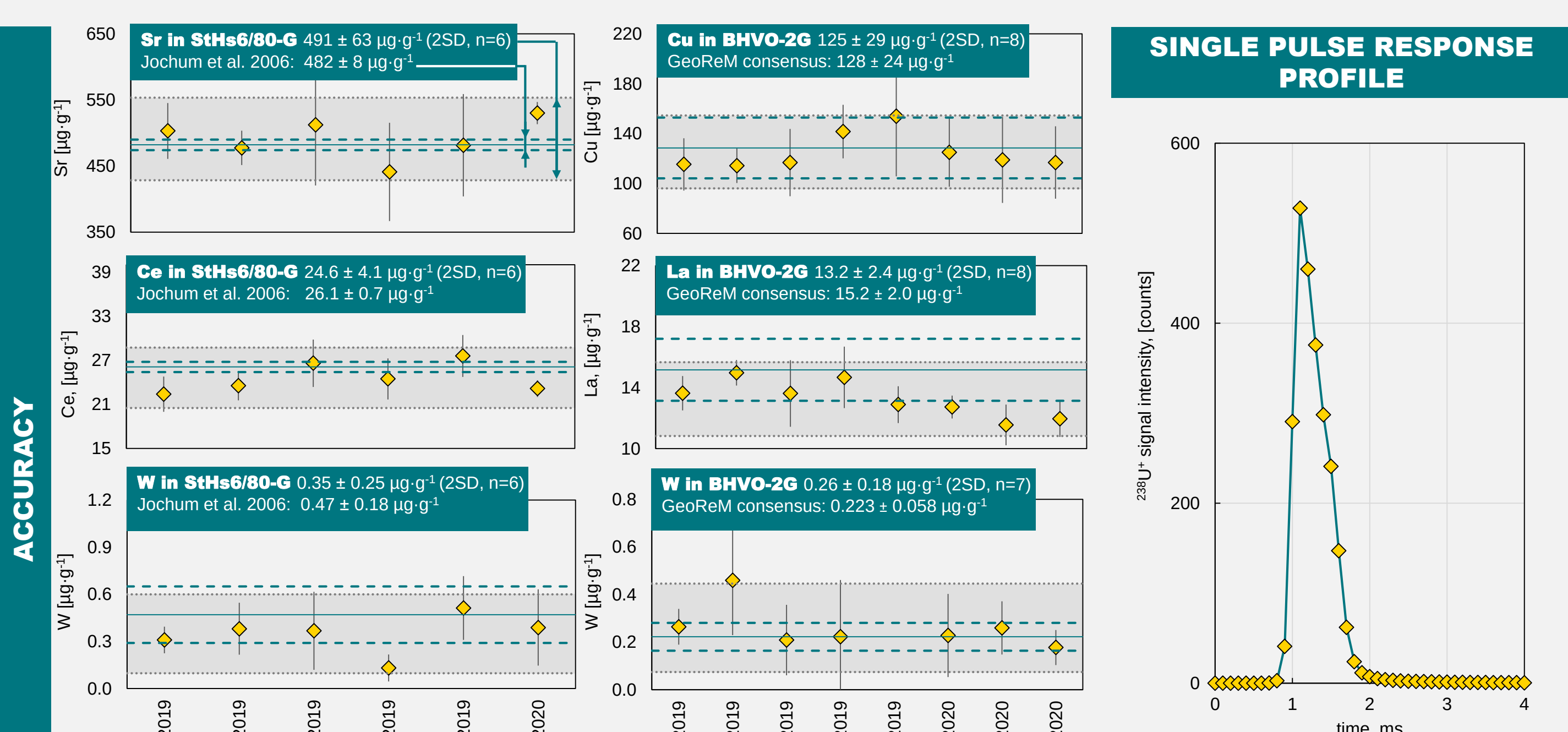
Fig. 5. Single pulse response profile of the LA-ICP-ToF-MS setup
