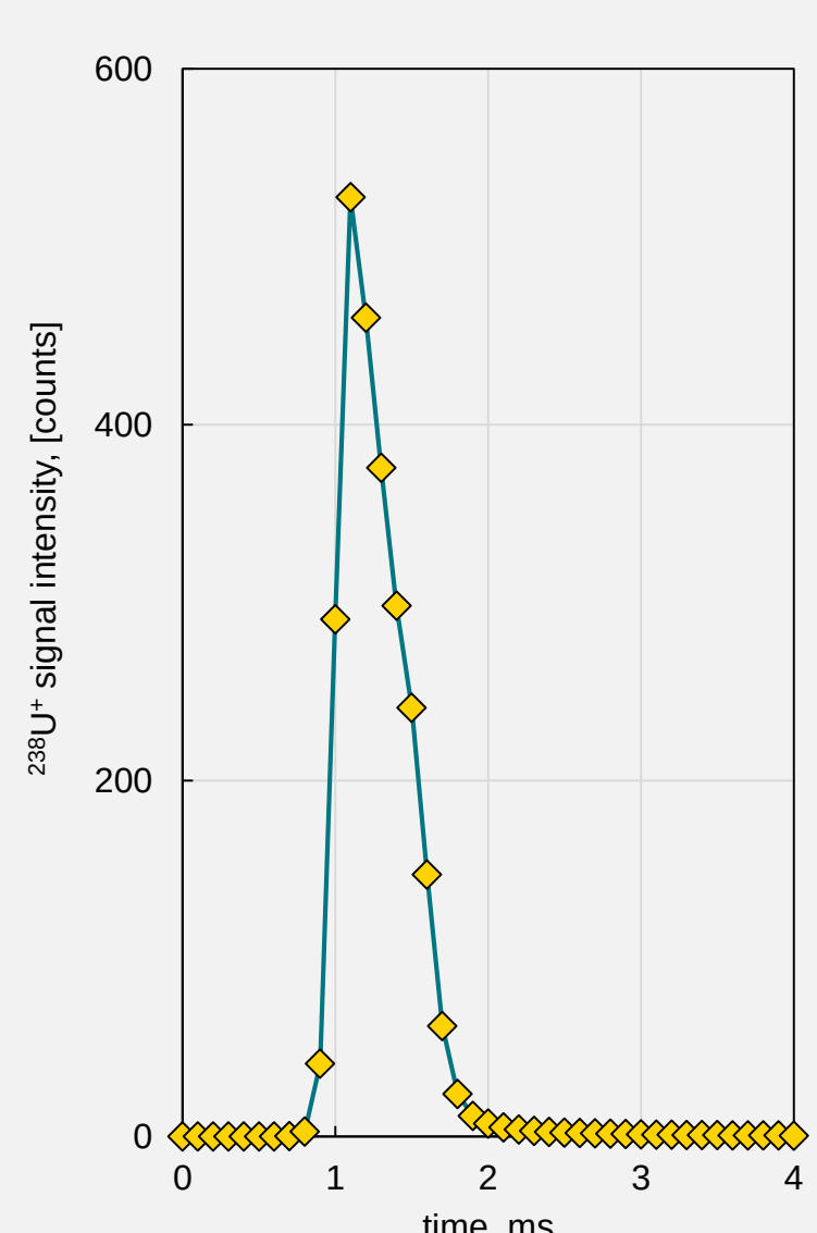
Fig. 5. Single pulse response profile of the LA-ICP-ToF-MS setup
